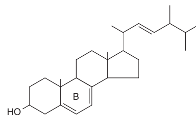
FIGURE 21-20 Ergosterol.
