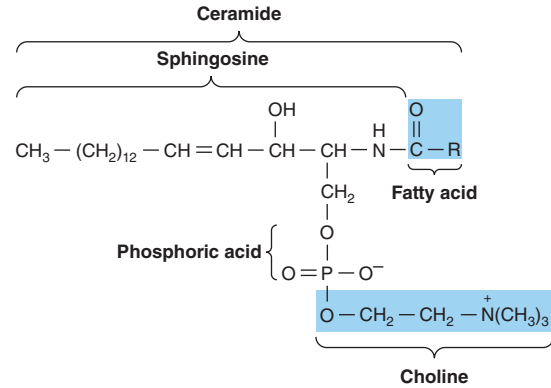
FIGURE 21-10 A sphingomyelin.
