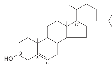
FIGURE 21-19 Cholesterol.
