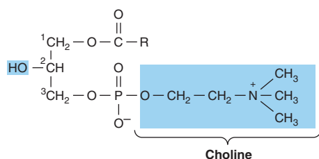
FIGURE 21-12 Lysophosphatidylcholine (lysolecithin).
