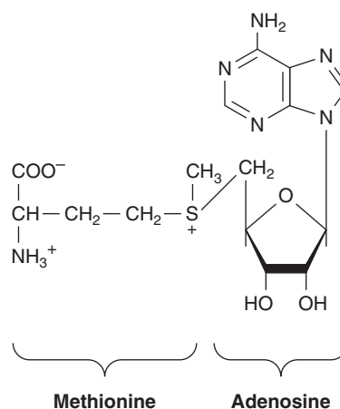
FIGURE 32-12 S -Adenosylmethionine.
