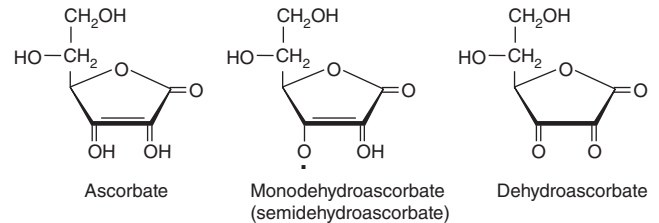
FIGURE 44–16 Vitamin C.
