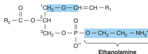
FIGURE 21-13 Plasmalogen.
