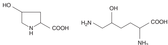
FIGURE 3-2 4-Hydroxyproline & 5-hydroxylysine.
